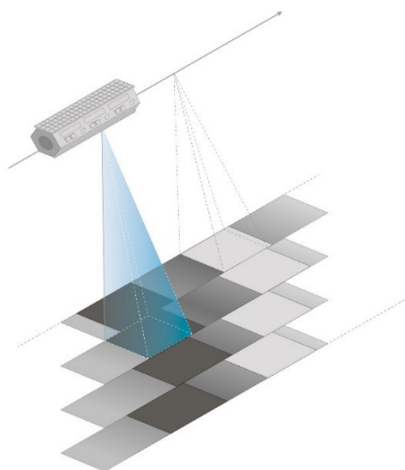
Figure 4 – ScanSAR mode acquisition geometry
